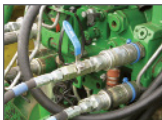
Ball valve wing lock up system
