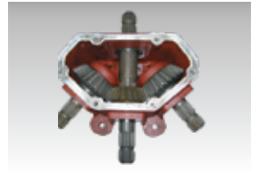
260hp heavy duty splitter box
