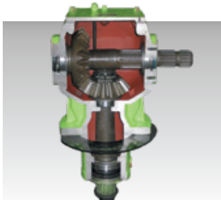
Heavy duty 210hp right angle gearboxes
