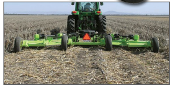
Can accommodate 30", 32" 38" 40" and 1 meter row spacing
